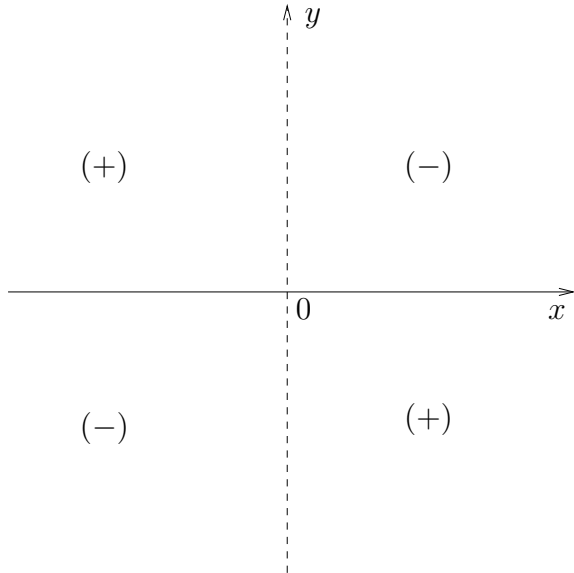
Fig. 2.2.1 Basic properties of the phase-plane for the linear harmonic oscillator. The dashed-line (- -) is the “zero” null-cline, the solid line (—) is the “infinite” null-cline. The (\pm) indicates the sign of dy/dx for the designated region.
