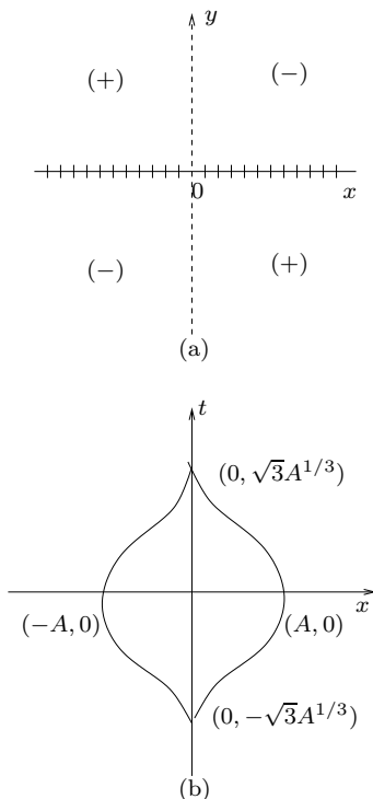
Fig. 3.2.1 (a) Phase-plane for \dot{x} + x^{-1/3} = 0 . Vertical dashes denote the infinite null-cline, y_\infty(x) . (b) Trajectory passing through x(0) = A and y(0) = 0 .
