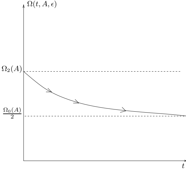
Fig. 7.4.1 Plot of \Omega(t, A, \epsilon) versus t , for the linearly damped, pure cubic Duffing equation. \Omega_0(A) = (\frac{3}{4})^{1/2} A .
