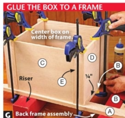
Position the box \frac{1}{4} " below the top edge of the middle rail. If you want the optional back (H), add it before attaching the front frame.
