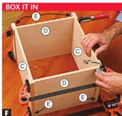
Glue the two L-shaped assemblies (C/D/E) together. Check for identical insets on both sides and for square.
