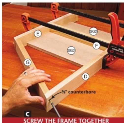
C SCREW THE FRAME TOGETHER
