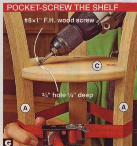
G First, using the shelf (C) shank holes as guides, drill pilot holes into the legs (A); then drive the screws.
