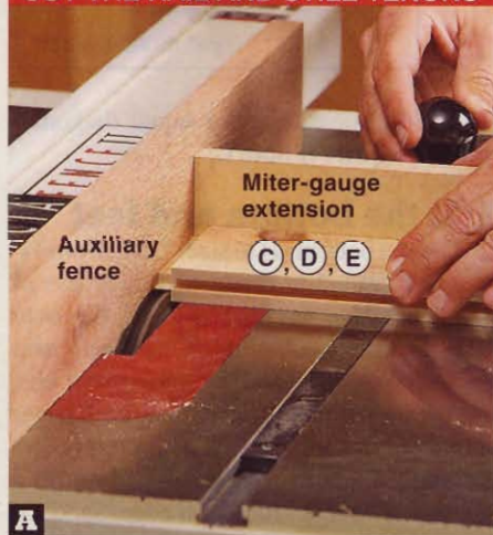
A Using a miter-gauge extension for backup, form a \frac{1}{4} " tenon \frac{3}{8} " long on each end of the rails (C, D) and center stiles (E).
