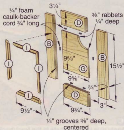
SIDE ASSEMBLY
