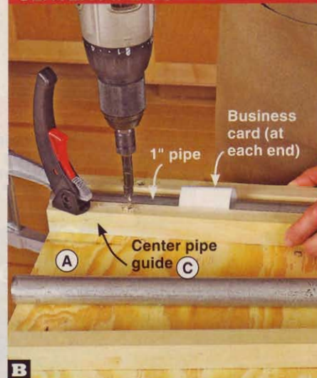
B With a business card bent around a 1" pipe at each end for a spacer, mount the center pipe guides (C) to the bottom platform (A).
