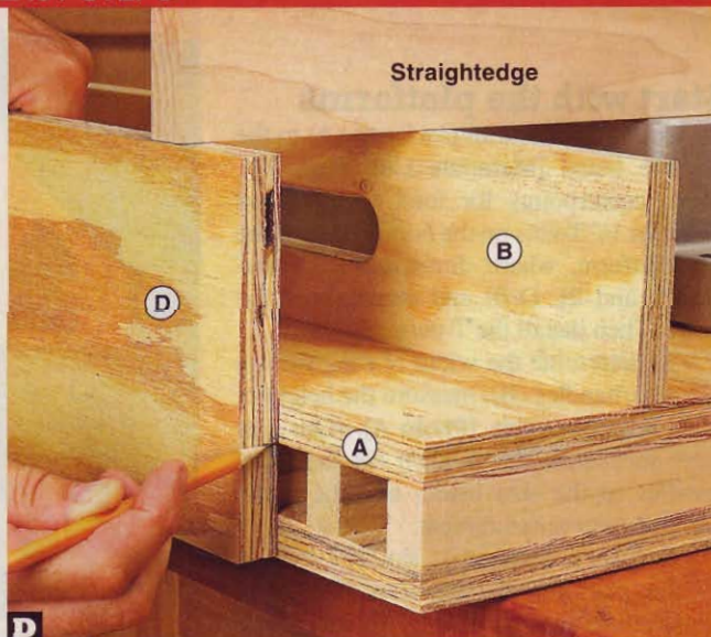
D Flip the rest up 90°. Then mark the location of the bottom of the top platform (A) on the end of the rest.
