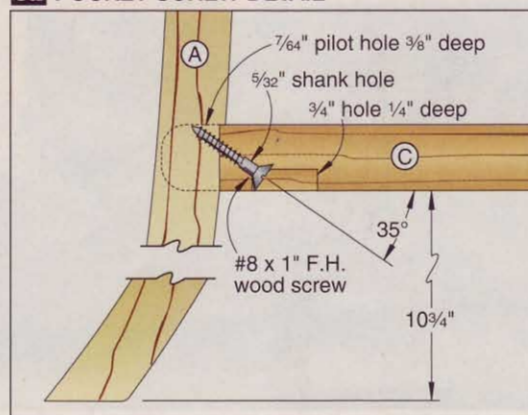
G First, using the shelf (C) shank holes as guides, drill pilot holes into the legs (A); then drive the screws.
