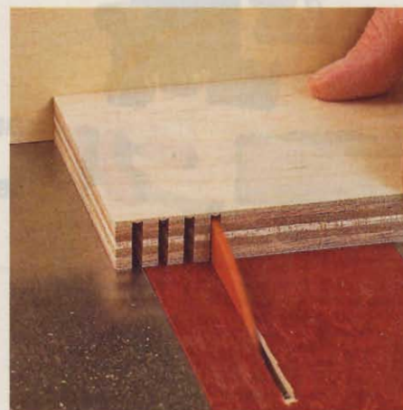
Dropping each successive saw kerf over the pin, kerf the entire length of the workpiece.
