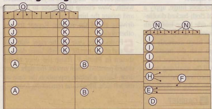
3/4 x 48 x 96" Baltic birch plywood
