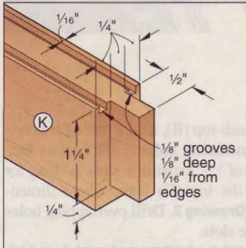
1a RAIL-TENON DETAIL
