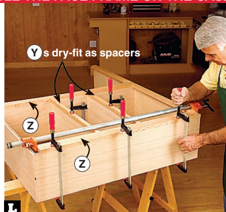
L Insert the short stiles (Y) as spacers between the upper and lower rails (Z). Then glue and clamp the upper rail in place.
