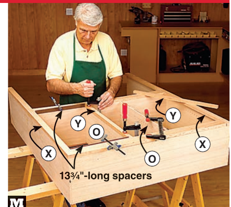
M Inserting 13\frac{3}{4} "-long spacers between the long stiles (X) and short stiles (Y), glue and clamp the short stiles to the dividers (O).
