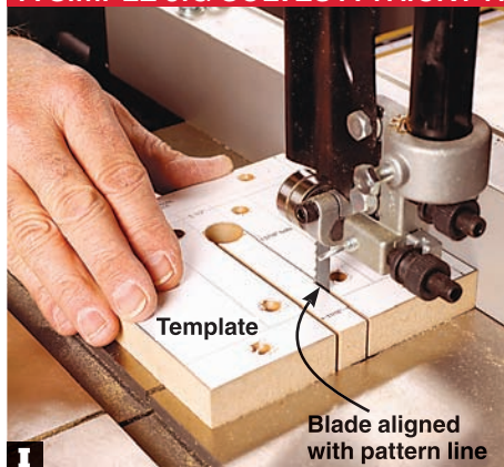
I Position your bandsaw fence to align the blade with the template pattern line, and saw along the lines into the \frac{1}{16} " hole.
