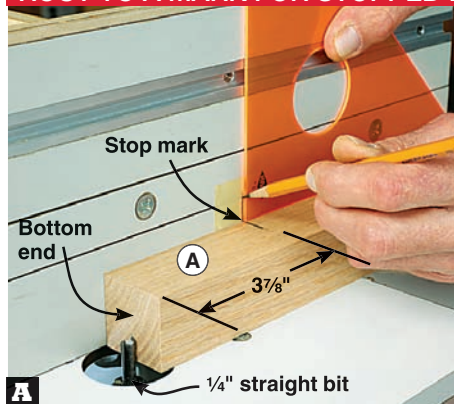
A With the end of the leg (A) against the right side of the bit, transfer the leg groove stop mark to a piece of masking tape on the fence.
