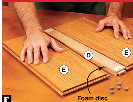
F With the muntin (D) centerlines facing up, place five foam discs in each muntin groove, and slide in the panels (E), bevels down.
