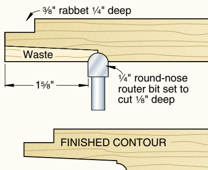
A \frac{1}{4} " round-nose bit creates a distinct panel.
