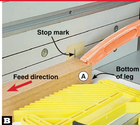
B Starting from the top end of each leg (A), rout the grooves, stopping when the bottom of the leg aligns with the mark on the fence.
