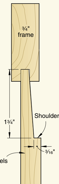
PROUD PANEL
