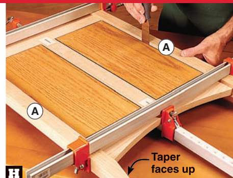
H Spread glue in the leg (A) mortises, and with end tapers facing up, clamp the legs in place. Center the panels with a putty knife.
