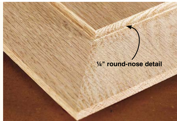
A \frac{1}{4} " round-nose bit creates a distinct panel.
