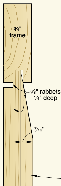
PLAIN-BEVEL PANEL
