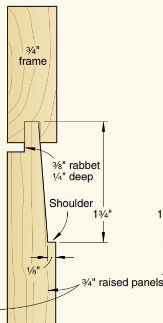
BACK-CUT PANEL
