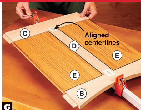
G Insert eight foam discs in each rail (B, C) groove. Apply glue to the muntin (D) tenons and add the rails, aligning the centerlines.
