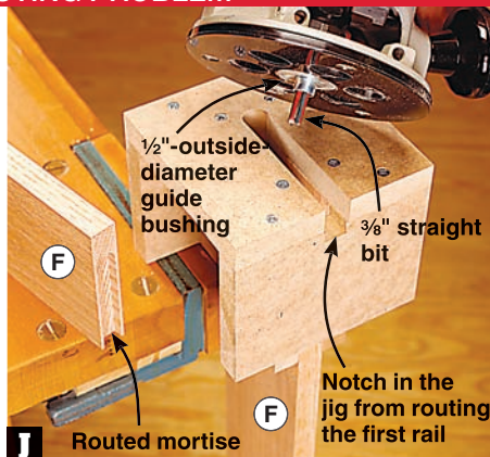
J Clamp a base rail (F) and jig in your bench vise. Running the guide bushing along the template slot edge, rout a \frac{1}{16} "-deep mortise.
