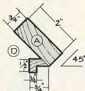
Cutting diagram
