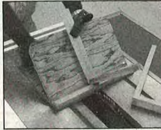
Cutting grooves with jig*
