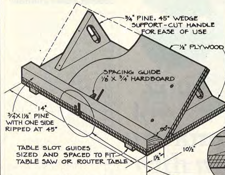
MULTI-FEATHER JOINT JIG WITH DETAIL FOR DOVETAIL KEY JIG
