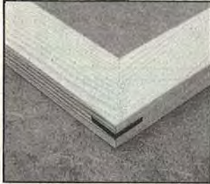
THROUGH SPLINE
