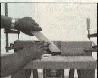
Cutting mortise with router*
