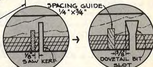
MULTI-FEATHER DOVETAIL KEY JIG
