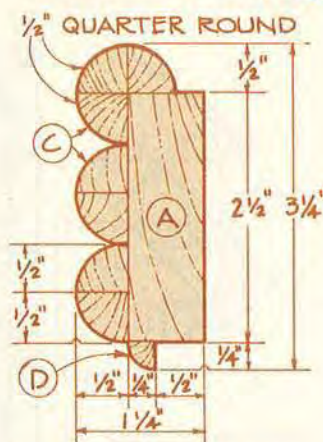
FRAME SECTION
