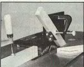
Cutting groove using stop block
