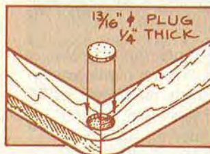
SURFACE SPLINE DETAIL
