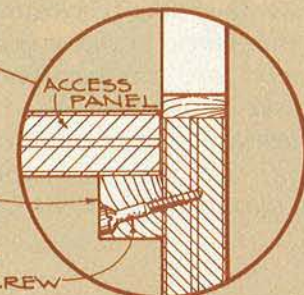
SIDE SECTION A-A
