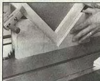
Cut groove with V-block jig
