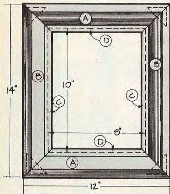
Cutting diagram
