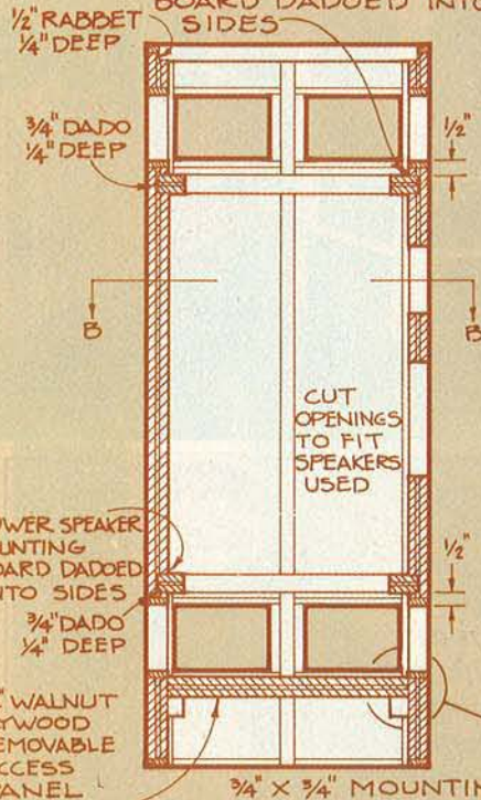
SIDE SECTION A-A
