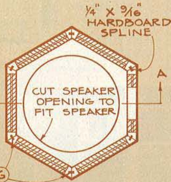
TOP SECTION B-B
